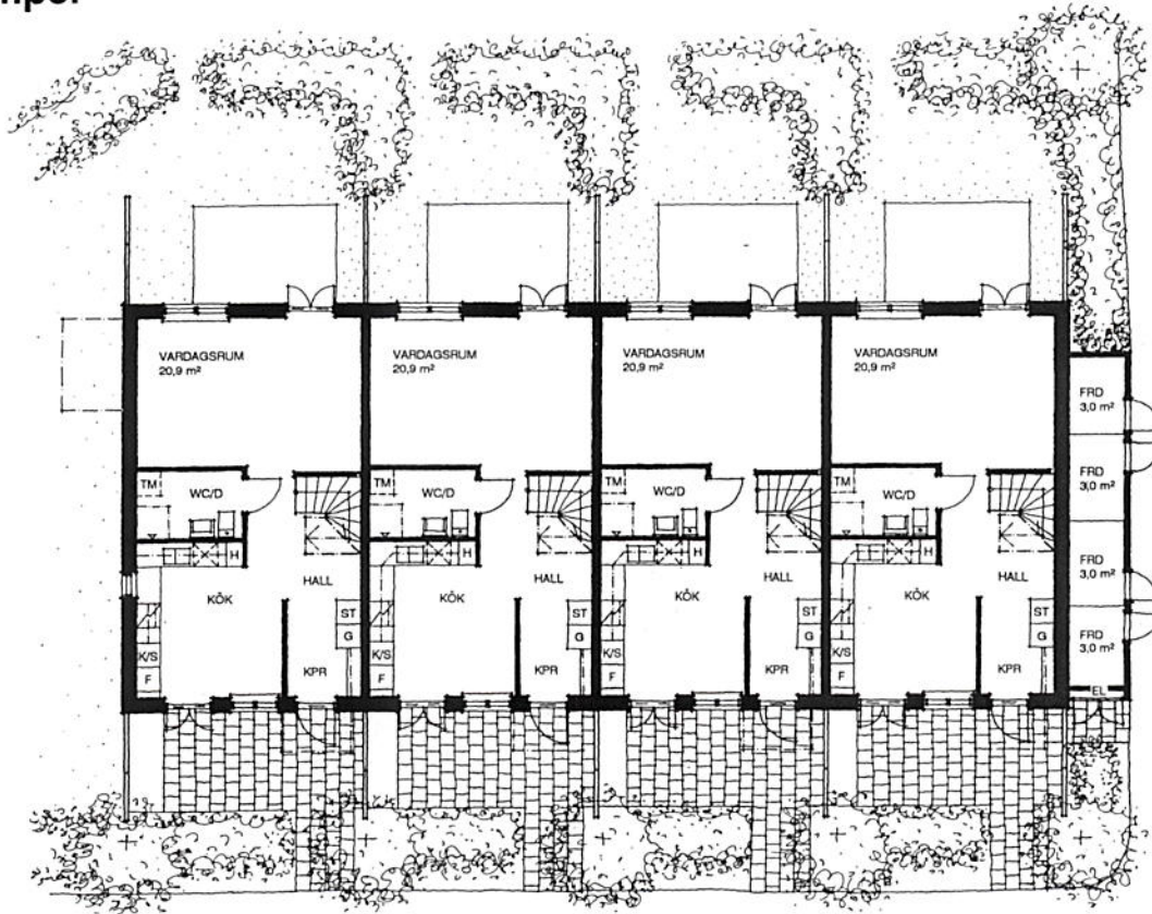
BOTTENPLAN
